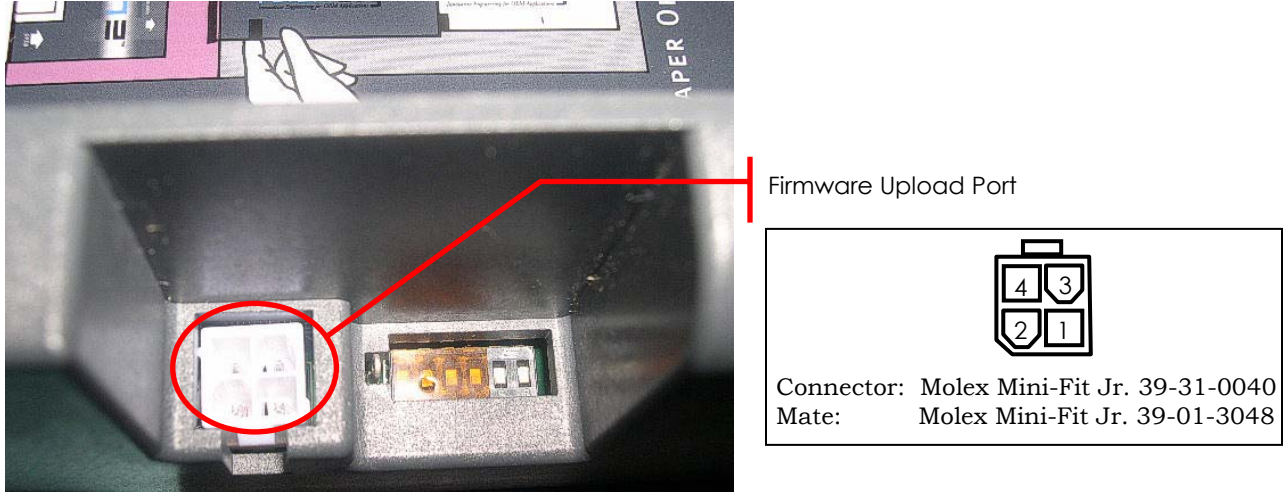
Figure 4-10 RS232 Firmware Upload Port
