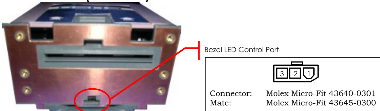
Figure 4-1 Front Bezel LED Control Port (All Models)
